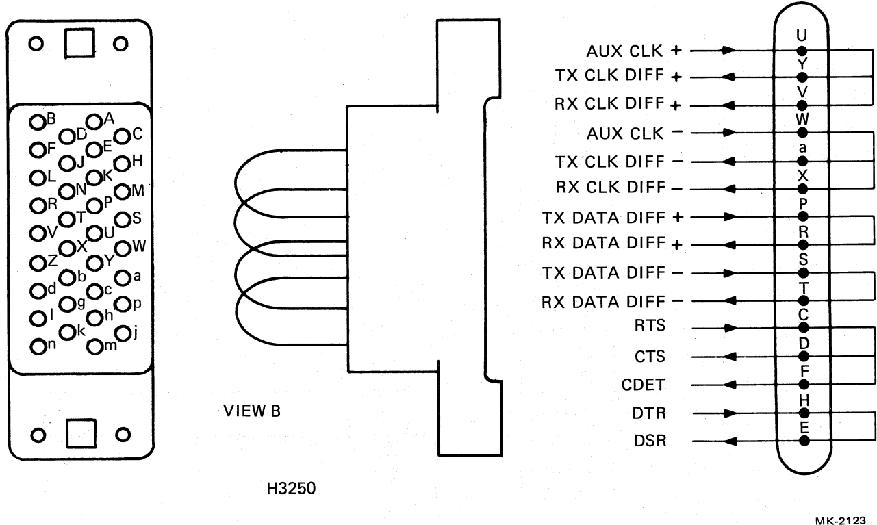
Figure 2-5 DMR11 Turnaround Test Connectors (Sheet 2 of 5)
