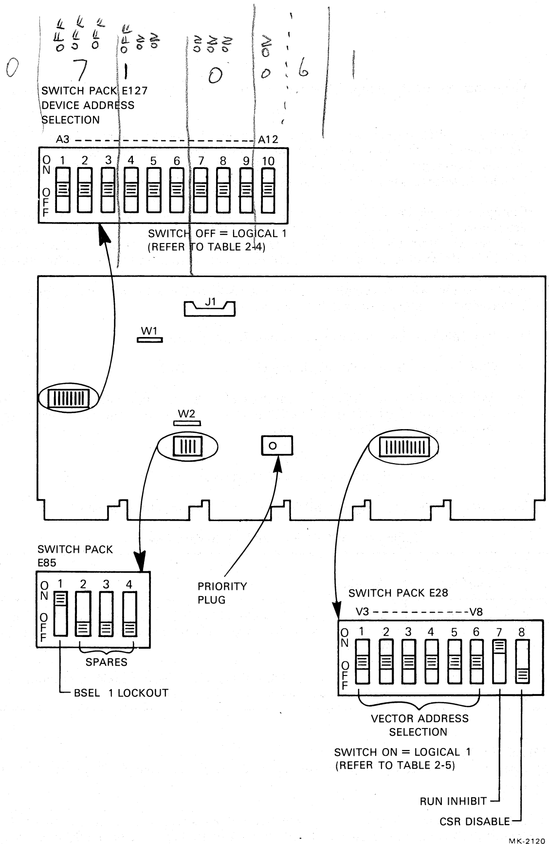
Figure 2-1 M8207-RA Microprocessor Switch/Jumper Locations
