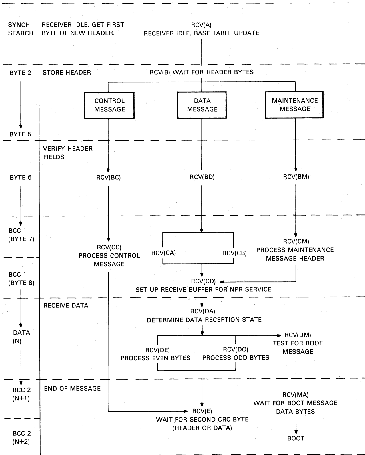
Figure D-5 Receive Process Flow Diagram
