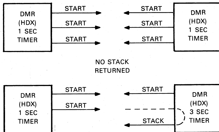
Figure 3-9 Start/Stack Sequence Timer
