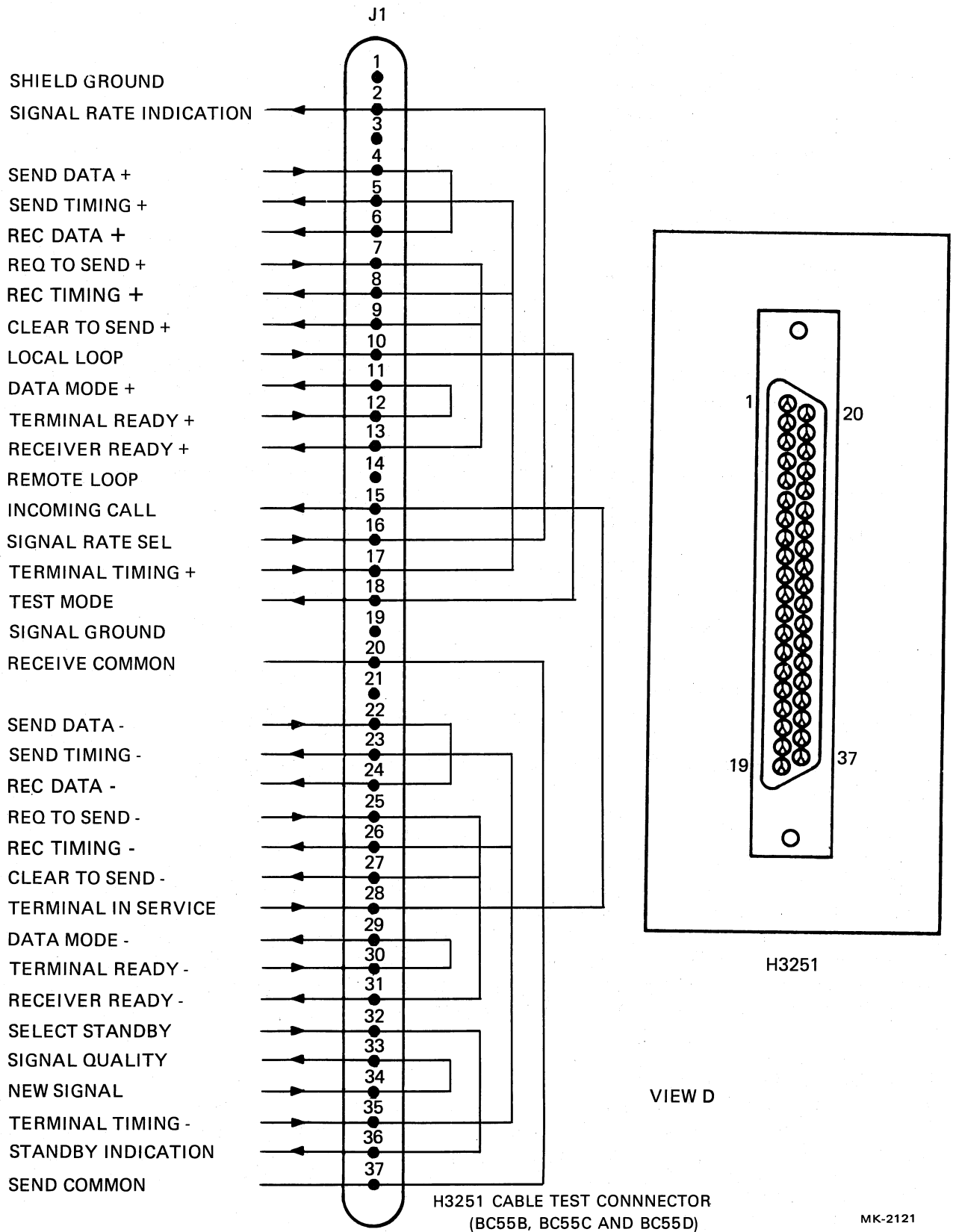
Figure 2-5 DMR11 Turnaround Test Connectors (Sheet 4 of 5)
